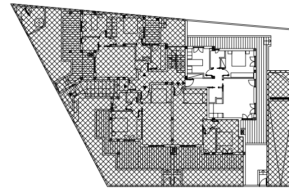
PIANO TERRENO
